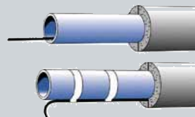
Internal and external installation of insulated pipes.
